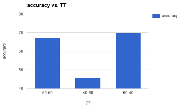
Figure 9. Accuracy
