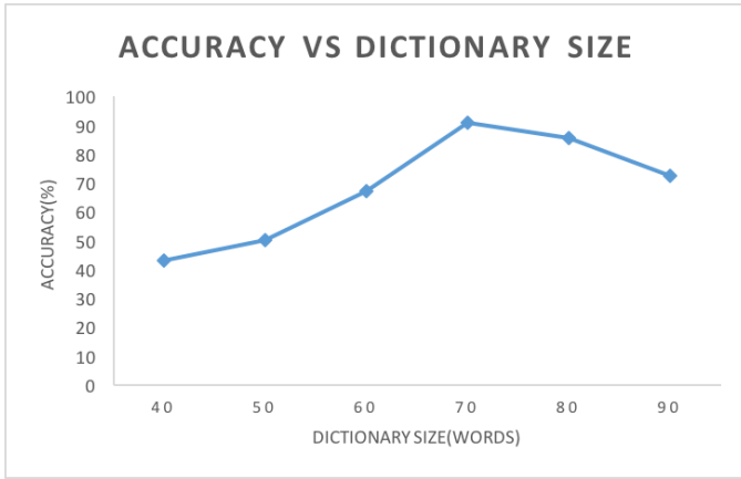
Figure 7. Accuracy
