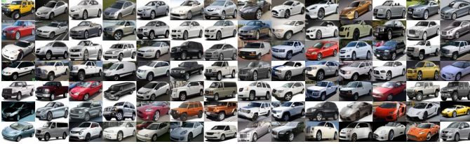
Figure 4. Car Dataset
