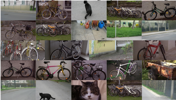
Figure 5. Non-Car Dataset
