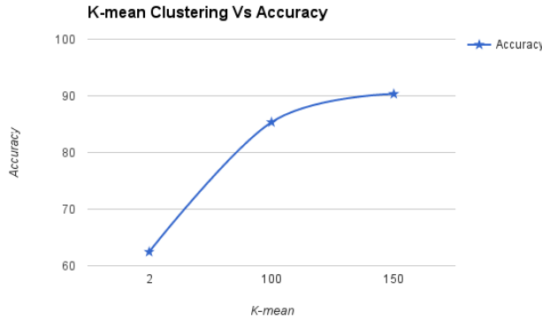
Figure 8. Accuracy
